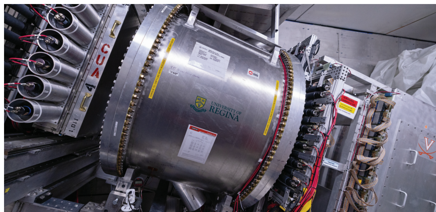
The SHMS detector stack inside Experimental Hall C at Jefferson Lab.
