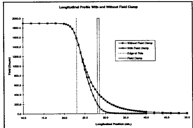
Figure 2: Longitudinal field fall-off with added field clamp.
