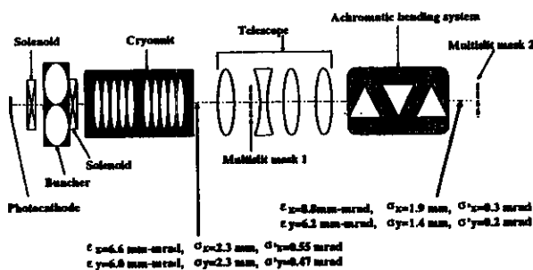
Figure 1: Schematic of the FEL injector. Normalized emittance, beam size and beam divergence at 135 pC bunch charge are given at the cryonit exit and the injection point according to PARMELA.
