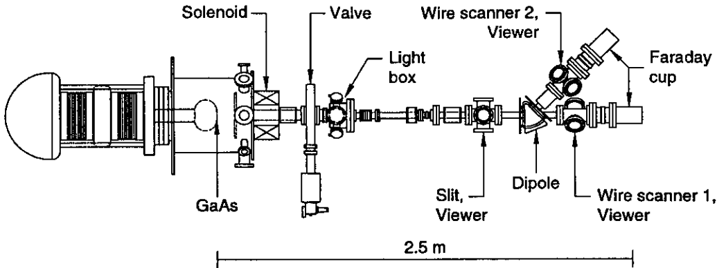
Figure 1: An overhead view of the gun (6 MV/m configuration) and the diagnostic beamline.
