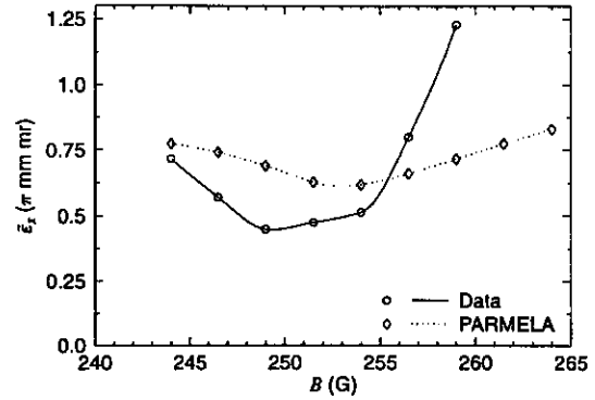
Figure 3: Results for measurements with R = 0.61 mm, \sigma_t = 20 ps, and q = 18.7 pC, showing the dependence of \bar{\epsilon}_x on B .
