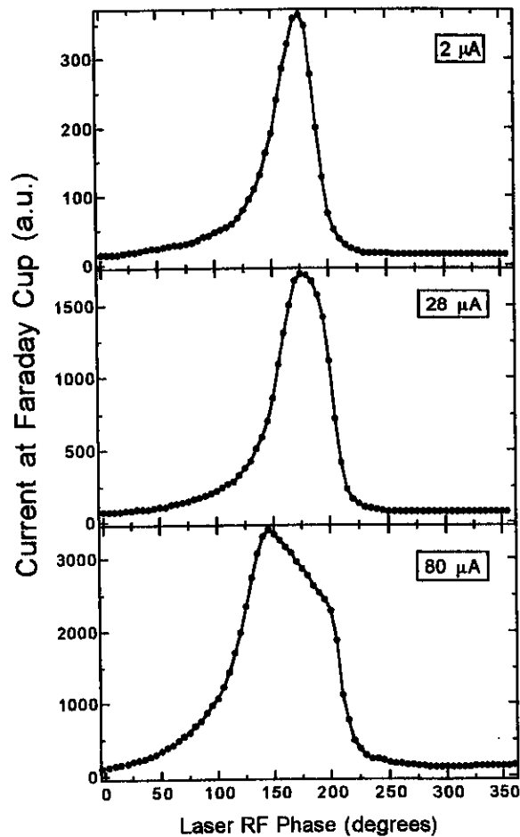
Figure 3. Electron bunch profiles for three different beam currents; 2, 28 and 80 \mu\text{A} .
