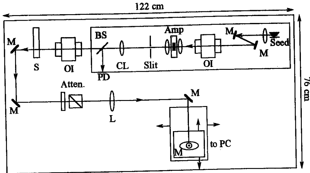
Figure 1. A schematic of the laser system. OI, optical isolator; S, shutter; M, mirror; PC, Pockels cell; CL, cylindrical lens; L, lens; BS, beam splitter.
