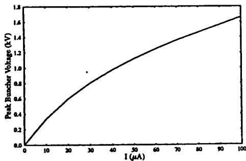
Figure 3 Calculated buncher voltage as a function of current (for an ideal, zero-length buncher).
