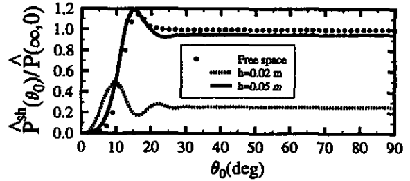
Figure 2: Transient power loss of a bunch, due to curvature-induced self-interaction in the presence of parallel plates, with \rho = 1 m, \sigma_s = 1 mm, and various plate spacings h . Here \theta_0 is the angle of bunch center into the bend.
