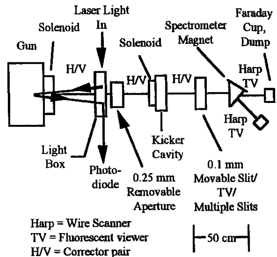
Figure 1. Schematic of the injector test stand.
