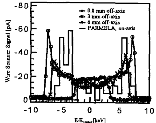
Figure 4. Plot of energy spread of beamlets sampled at 0.8, 3.0, and 6.0 mm off-axis. The profile generated by PARMELA simulation is derived from particles within 0.5 mm of the beam axis.
