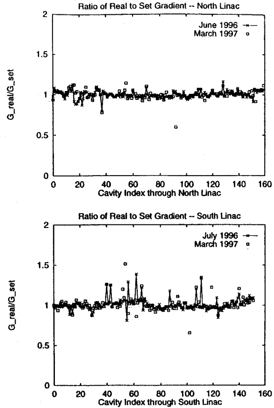
Figure 2: Measured Gradient ratio comparison from June/July, 1996, to March, 1997, for the North and South Linacs at CEBAF. Note the persistence of fine structure over the nine month interval between measurements.
