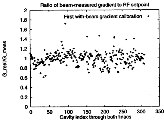
Figure 1: First measurement of linac gradient errors
