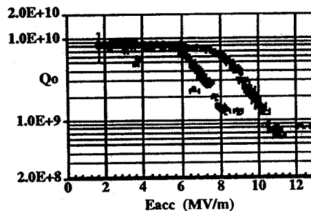
Figure 3 IA174 vertical test data that resulted in a ceramic puncture.
