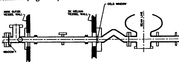
Figure 4 Dogleg Fundamental Power Coupler
