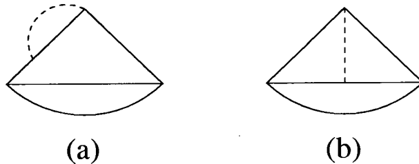
FIG. 1. Perturbative diagrams. Dashed line denotes gluon. (Permutations are not shown)
