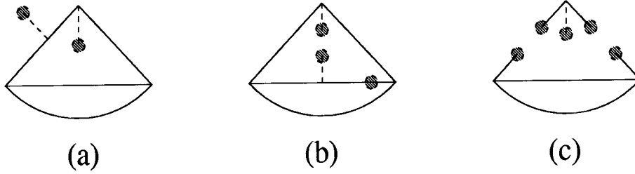
FIG. 2. Dimension-4 power corrections: local (a,b) and bilocal (c). Shaded circles mark vacuum fields
