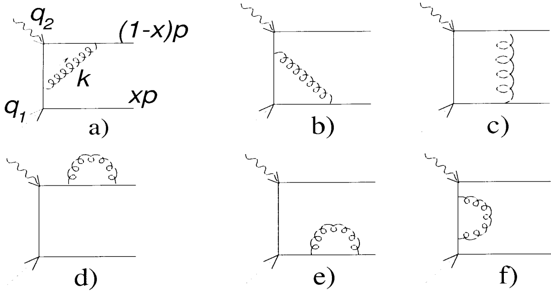
FIG. 3. One-loop diagrams.
