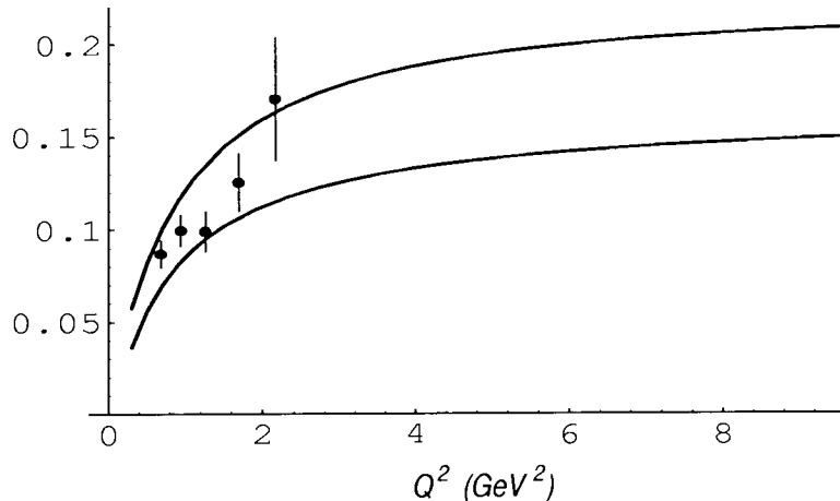
FIG. 4. Combination \sqrt{2}Q^2 F_{\gamma^* \gamma \pi^0}(Q^2)/4\pi (measured in GeV and equivalent to Q^2 \tilde{F}_{\gamma^* \gamma \pi^0}(Q^2) , with the form factor \tilde{F}_{\gamma^* \gamma \pi^0}(Q^2) normalized according to definition adopted in refs.[21,26,38]) as a function of Q^2 . The lower curve corresponds to our model with the asymptotic DA (Eq.(5.45)) and the upper one is based on Eq.(5.46). Data are taken from CELLO collaboration publication [14]. Preliminary CLEO data [15] (not shown) are very close to the lower curve.
