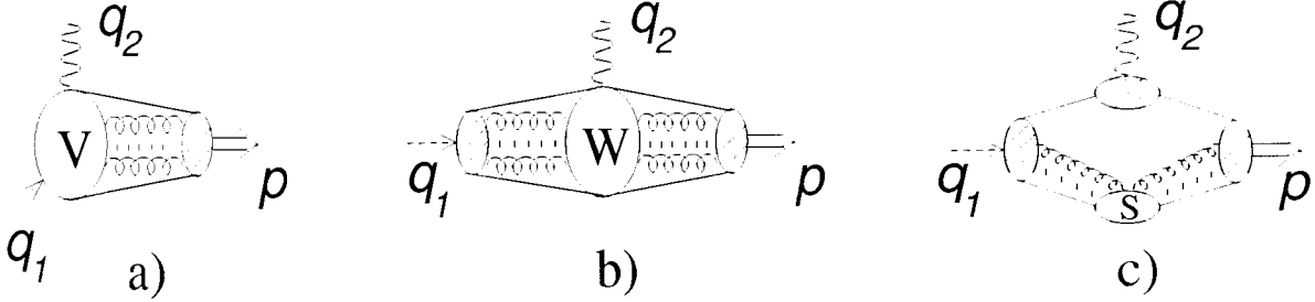
FIG. 1. Structure of factorization for the F_{\gamma^*\gamma\pi^0}(Q^2) form factor at large Q^2 .
