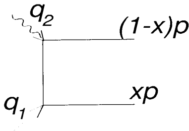
FIG. 2. Lowest-order diagram.
