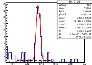
\pi^0 angle: [0.70, 0.80] elasticity: [1.15, 1.16]
