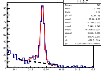
\pi^0 angle: [0.50, 0.60] elasticity: [0.89, 0.91]
