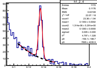
\pi^0 angle: [0.20, 0.30] elasticity: [0.85, 0.87]
