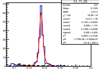
\pi^0 angle: [1.10, 1.20] elasticity: [1.07, 1.08]
