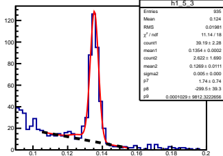
\pi^0 angle: [0.50, 0.60] elasticity: [0.84, 0.85]
