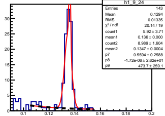
\pi^0 angle: [0.90, 1.00] elasticity: [1.12, 1.13]
