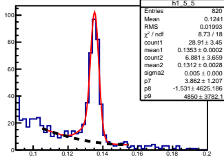
\pi^0 angle: [0.50, 0.60] elasticity: [0.87, 0.88]
