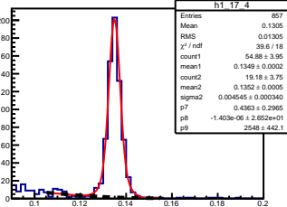
\pi^0 angle: [1.70, 1.80] elasticity: [0.85, 0.87]
