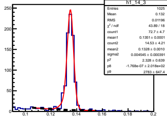
\pi^0 angle: [1.40, 1.50] elasticity: [0.84, 0.85]
