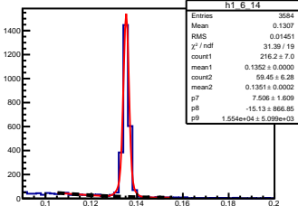
\pi^0 angle: [0.60, 0.70] elasticity: [0.99, 1.00]
