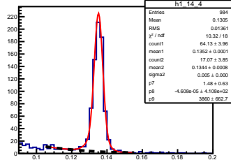
\pi^0 angle: [1.40, 1.50] elasticity: [0.85, 0.87]
