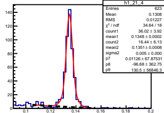
\pi^0 angle: [2.10, 2.20] elasticity: [0.85, 0.87]
