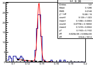
\pi^0 angle: [0.90, 1.00] elasticity: [1.15, 1.16]
