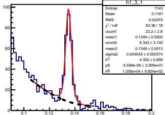
\pi^0 angle: [0.30, 0.40] elasticity: [0.81, 0.83]
