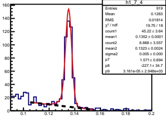
\pi^0 angle: [0.70, 0.80] elasticity: [0.85, 0.87]
