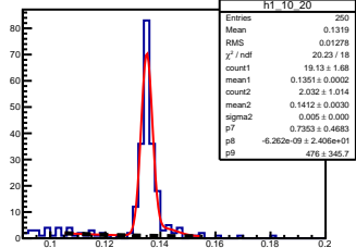
\pi^0 angle: [1.00, 1.10] elasticity: [1.07, 1.08]
