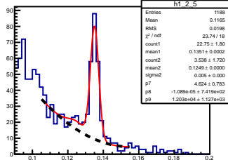
\pi^0 angle: [0.20, 0.30] elasticity: [0.87, 0.88]
