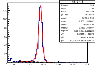
\pi^0 angle: [2.10, 2.20] elasticity: [0.91, 0.92]
