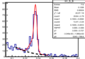
\pi^0 angle: [0.50, 0.60] elasticity: [0.91, 0.92]
