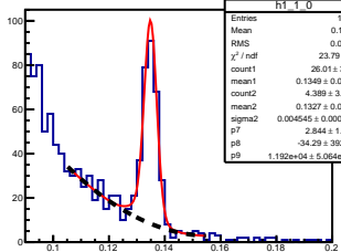
\pi^0 angle: [0.10, 0.20] elasticity: [0.80, 0.81]
