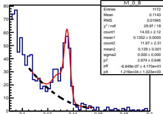
\pi^0 angle: [0.00, 0.10] elasticity: [0.91, 0.92]
