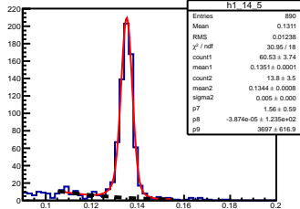
\pi^0 angle: [1.40, 1.50] elasticity: [0.87, 0.88]
