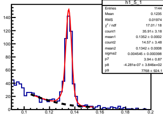
\pi^0 angle: [0.50, 0.60] elasticity: [0.81, 0.83]
