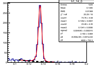
\pi^0 angle: [1.40, 1.50] elasticity: [0.80, 0.81]
