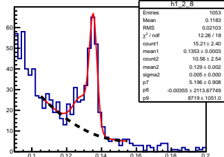
\pi^0 angle: [0.20, 0.30] elasticity: [0.91, 0.92]
