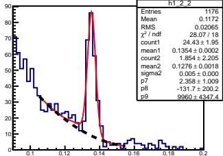
\pi^0 angle: [0.20, 0.30] elasticity: [0.83, 0.84]
