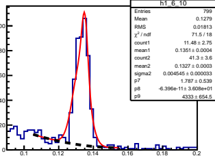
\pi^0 angle: [0.60, 0.70] elasticity: [0.93, 0.95]
