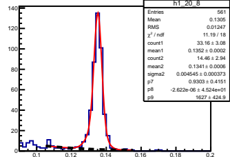
\pi^0 angle: [2.00, 2.10] elasticity: [0.91, 0.92]
