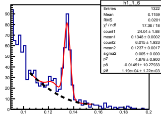
\pi^0 angle: [0.10, 0.20] elasticity: [0.88, 0.89]
