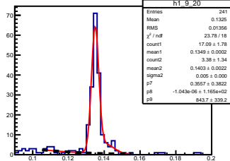
\pi^0 angle: [0.90, 1.00] elasticity: [1.07, 1.08]
