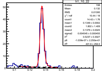
\pi^0 angle: [1.00, 1.10] elasticity: [1.09, 1.11]
