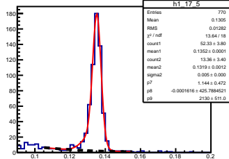
\pi^0 angle: [1.70, 1.80] elasticity: [0.87, 0.88]
