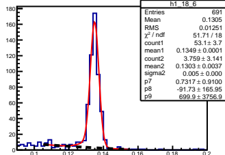
\pi^0 angle: [1.80, 1.90] elasticity: [0.88, 0.89]
