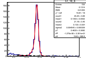
\pi^0 angle: [1.80, 1.90] elasticity: [0.91, 0.92]
