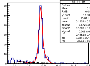
\pi^0 angle: [1.10, 1.20] elasticity: [1.05, 1.07]
