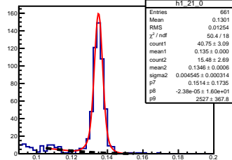
\pi^0 angle: [2.10, 2.20] elasticity: [0.80, 0.81]
