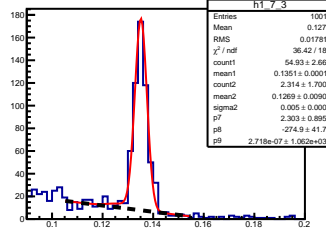
\pi^0 angle: [0.70, 0.80] elasticity: [0.84, 0.85]
