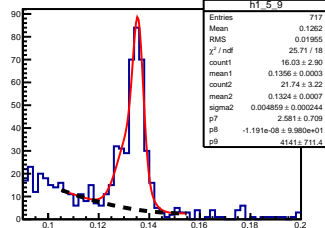
\pi^0 angle: [0.50, 0.60] elasticity: [0.92, 0.93]
