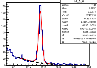
\pi^0 angle: [0.50, 0.60] elasticity: [0.80, 0.81]
