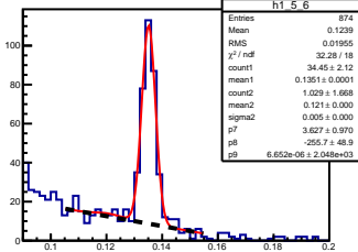
\pi^0 angle: [0.50, 0.60] elasticity: [0.88, 0.89]
