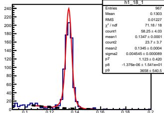
\pi^0 angle: [1.80, 1.90] elasticity: [0.81, 0.83]
