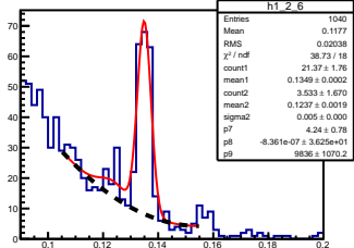
\pi^0 angle: [0.20, 0.30] elasticity: [0.88, 0.89]
