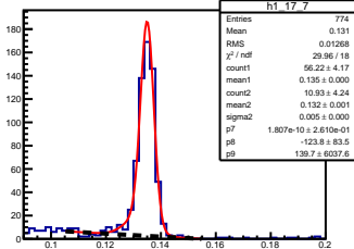
\pi^0 angle: [1.70, 1.80] elasticity: [0.89, 0.91]
