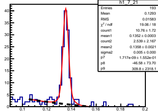
\pi^0 angle: [0.70, 0.80] elasticity: [1.08, 1.09]
