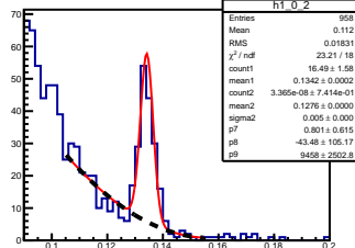
\pi^0 angle: [0.00, 0.10] elasticity: [0.83, 0.84]
