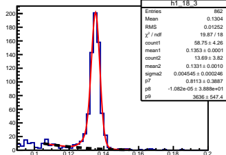
\pi^0 angle: [1.80, 1.90] elasticity: [0.84, 0.85]
