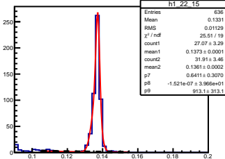
\pi^0 angle: [2.20, 2.30] elasticity: [1.00, 1.01]
