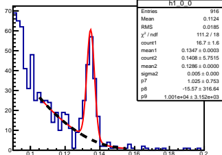
\pi^0 angle: [0.00, 0.10] elasticity: [0.80, 0.81]
