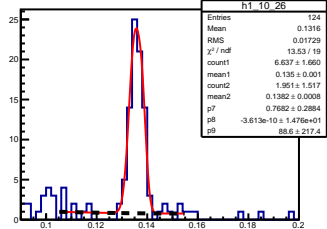
\pi^0 angle: [1.00, 1.10] elasticity: [1.15, 1.16]
