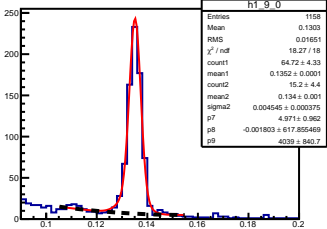
\pi^0 angle: [0.90, 1.00] elasticity: [0.80, 0.81]
