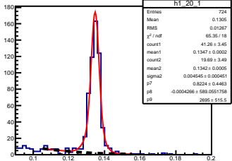
\pi^0 angle: [2.00, 2.10] elasticity: [0.81, 0.83]
