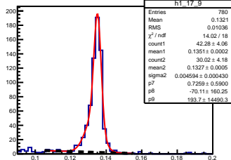
\pi^0 angle: [1.70, 1.80] elasticity: [0.92, 0.93]
