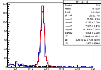
\pi^0 angle: [2.10, 2.20] elasticity: [0.87, 0.88]
