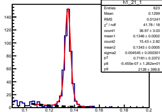
\pi^0 angle: [2.10, 2.20] elasticity: [0.81, 0.83]
