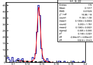
\pi^0 angle: [0.90, 1.00] elasticity: [1.09, 1.11]
