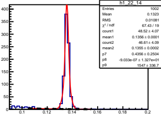
\pi^0 angle: [2.20, 2.30] elasticity: [0.99, 1.00]
