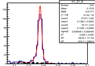
\pi^0 angle: [2.10, 2.20] elasticity: [0.92, 0.93]
