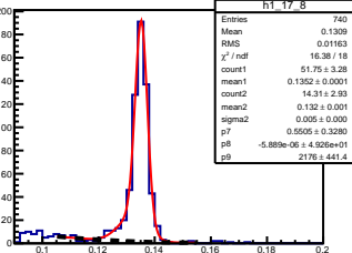
\pi^0 angle: [1.70, 1.80] elasticity: [0.91, 0.92]
