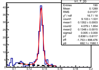
\pi^0 angle: [0.70, 0.80] elasticity: [1.07, 1.08]
