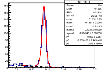
\pi^0 angle: [1.80, 1.90] elasticity: [0.85, 0.87]
