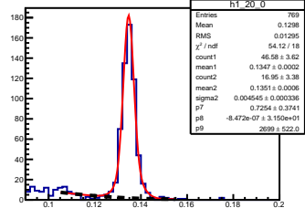
\pi^0 angle: [2.00, 2.10] elasticity: [0.80, 0.81]
