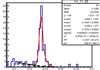
\pi^0 angle: [1.10, 1.20] elasticity: [1.17, 1.19]
