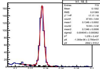
\pi^0 angle: [1.80, 1.90] elasticity: [0.87, 0.88]
