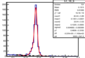
\pi^0 angle: [1.80, 1.90] elasticity: [0.92, 0.93]
