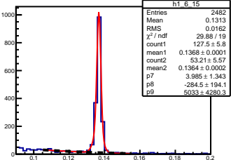
\pi^0 angle: [0.60, 0.70] elasticity: [1.00, 1.01]
