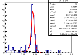
\pi^0 angle: [0.90, 1.00] elasticity: [1.17, 1.19]
