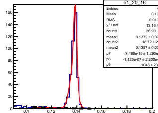
\pi^0 angle: [2.00, 2.10] elasticity: [1.01, 1.03]
