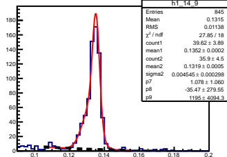
\pi^0 angle: [1.40, 1.50] elasticity: [0.92, 0.93]
