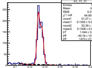
\pi^0 angle: [1.10, 1.20] elasticity: [0.95, 0.96]
