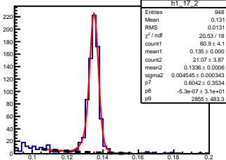
\pi^0 angle: [1.70, 1.80] elasticity: [0.83, 0.84]
