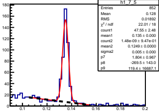
\pi^0 angle: [0.70, 0.80] elasticity: [0.87, 0.88]
