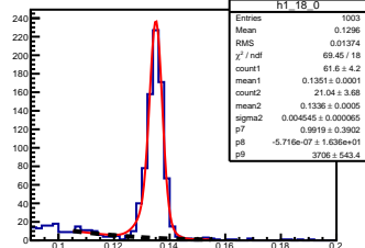
\pi^0 angle: [1.80, 1.90] elasticity: [0.80, 0.81]
