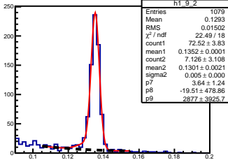
\pi^0 angle: [0.90, 1.00] elasticity: [0.83, 0.84]
