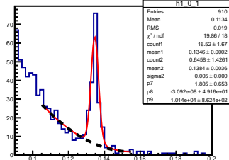
\pi^0 angle: [0.00, 0.10] elasticity: [0.81, 0.82]
