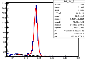
\pi^0 angle: [1.40, 1.50] elasticity: [0.88, 0.89]
