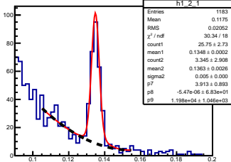
\pi^0 angle: [0.20, 0.30] elasticity: [0.81, 0.83]
