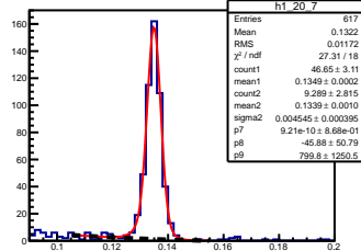
\pi^0 angle: [2.00, 2.10] elasticity: [0.89, 0.91]
