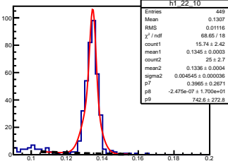
\pi^0 angle: [2.20, 2.30] elasticity: [0.93, 0.95]
