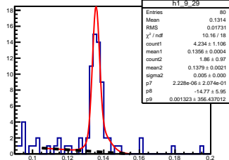
\pi^0 angle: [0.90, 1.00] elasticity: [1.19, 1.20]
