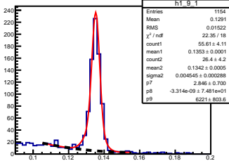
\pi^0 angle: [0.90, 1.00] elasticity: [0.81, 0.83]
