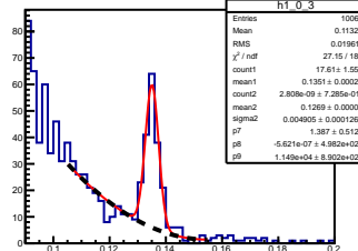
\pi^0 angle: [0.00, 0.10] elasticity: [0.84, 0.85]
