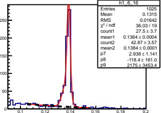
\pi^0 angle: [0.60, 0.70] elasticity: [1.01, 1.03]
