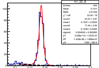
\pi^0 angle: [2.20, 2.30] elasticity: [0.91, 0.92]
