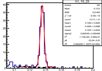
\pi^0 angle: [1.00, 1.10] elasticity: [1.11, 1.12]
