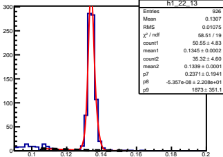
\pi^0 angle: [2.20, 2.30] elasticity: [0.97, 0.99]
