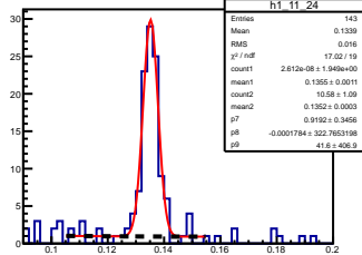
\pi^0 angle: [1.10, 1.20] elasticity: [1.12, 1.13]
