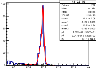
\pi^0 angle: [2.20, 2.30] elasticity: [1.01, 1.03]
