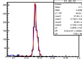
\pi^0 angle: [2.00, 2.10] elasticity: [0.96, 0.97]
