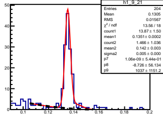
\pi^0 angle: [0.90, 1.00] elasticity: [1.08, 1.09]
