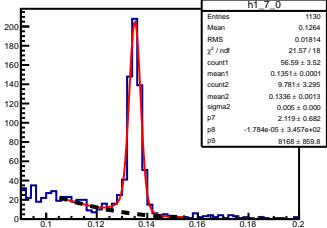
\pi^0 angle: [0.70, 0.80] elasticity: [0.80, 0.81]
