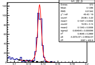
\pi^0 angle: [2.20, 2.30] elasticity: [0.80, 0.81]
