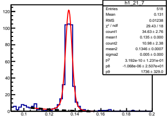
\pi^0 angle: [2.10, 2.20] elasticity: [0.89, 0.91]
