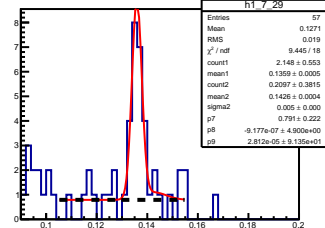
\pi^0 angle: [0.70, 0.80] elasticity: [1.19, 1.20]
