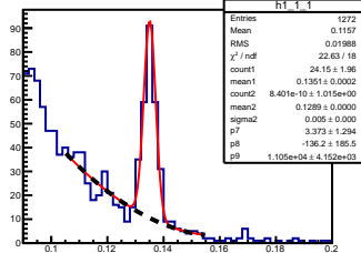
\pi^0 angle: [0.10, 0.20] elasticity: [0.81, 0.83]
