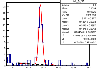
\pi^0 angle: [0.90, 1.00] elasticity: [1.16, 1.17]
