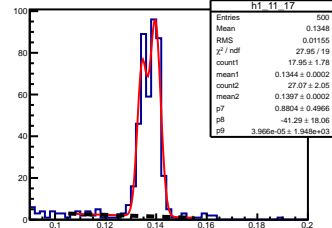
\pi^0 angle: [1.10, 1.20] elasticity: [1.03, 1.04]
