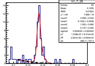
\pi^0 angle: [0.70, 0.80] elasticity: [1.17, 1.19]
