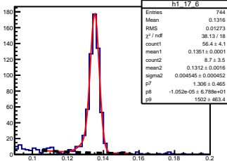
\pi^0 angle: [1.70, 1.80] elasticity: [0.88, 0.89]
