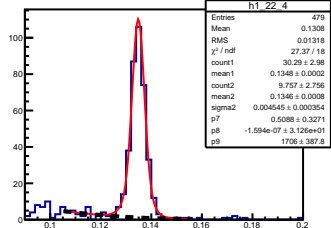
\pi^0 angle: [2.20, 2.30] elasticity: [0.85, 0.87]
