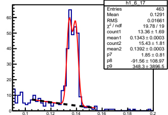
\pi^0 angle: [0.60, 0.70] elasticity: [1.03, 1.04]
