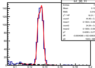
\pi^0 angle: [2.00, 2.10] elasticity: [0.95, 0.96]
