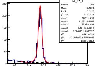
\pi^0 angle: [1.70, 1.80] elasticity: [0.81, 0.83]
