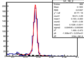
\pi^0 angle: [1.80, 1.90] elasticity: [0.83, 0.84]
