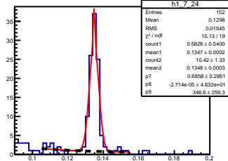
\pi^0 angle: [0.70, 0.80] elasticity: [1.12, 1.13]
