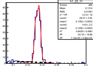
\pi^0 angle: [2.20, 2.30] elasticity: [0.95, 0.96]
