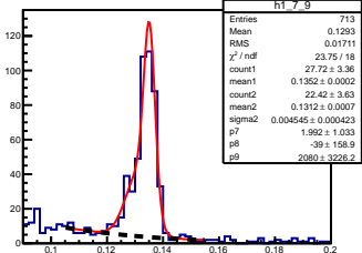
\pi^0 angle: [0.70, 0.80] elasticity: [0.92, 0.93]
