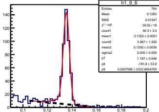
\pi^0 angle: [0.90, 1.00] elasticity: [0.88, 0.89]
