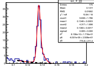
\pi^0 angle: [0.70, 0.80] elasticity: [1.09, 1.11]
