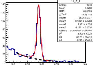
\pi^0 angle: [0.50, 0.60] elasticity: [0.83, 0.84]
