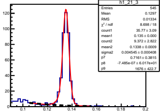
\pi^0 angle: [2.10, 2.20] elasticity: [0.84, 0.85]
