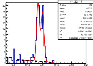
\pi^0 angle: [2.20, 2.30] elasticity: [1.03, 1.04]
