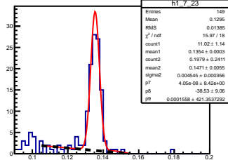
\pi^0 angle: [0.70, 0.80] elasticity: [1.11, 1.12]
