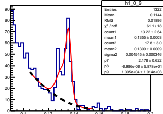
\pi^0 angle: [0.00, 0.10] elasticity: [0.92, 0.93]
