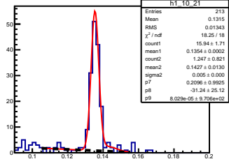
\pi^0 angle: [1.00, 1.10] elasticity: [1.08, 1.09]
