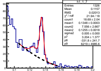
\pi^0 angle: [0.10, 0.20] elasticity: [0.89, 0.91]
