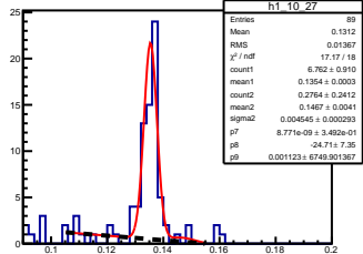
\pi^0 angle: [1.00, 1.10] elasticity: [1.16, 1.17]
