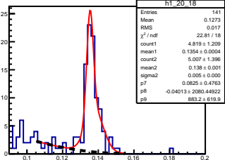
\pi^0 angle: [2.00, 2.10] elasticity: [1.04, 1.05]
