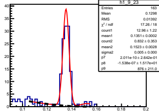
\pi^0 angle: [0.90, 1.00] elasticity: [1.11, 1.12]
