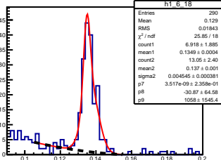
\pi^0 angle: [0.60, 0.70] elasticity: [1.04, 1.05]
