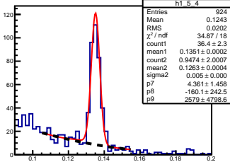
\pi^0 angle: [0.50, 0.60] elasticity: [0.85, 0.87]
