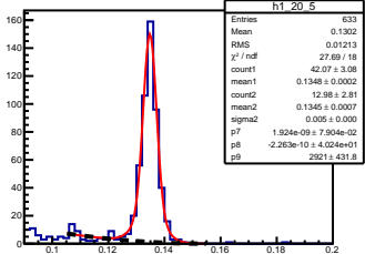
\pi^0 angle: [2.00, 2.10] elasticity: [0.87, 0.88]
