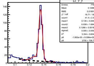
\pi^0 angle: [0.70, 0.80] elasticity: [0.89, 0.91]
