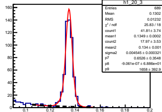
\pi^0 angle: [2.00, 2.10] elasticity: [0.84, 0.85]
