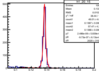
\pi^0 angle: [2.00, 2.10] elasticity: [1.00, 1.01]
