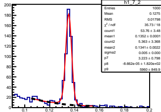
\pi^0 angle: [0.70, 0.80] elasticity: [0.83, 0.84]
