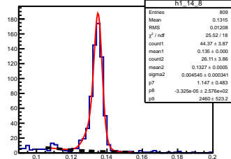
\pi^0 angle: [1.40, 1.50] elasticity: [0.91, 0.92]
