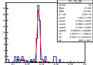
\pi^0 angle: [1.00, 1.10] elasticity: [1.19, 1.20]
