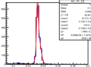
\pi^0 angle: [1.10, 1.20] elasticity: [0.96, 0.97]
