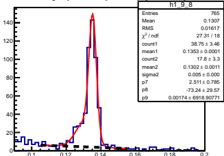
\pi^0 angle: [0.90, 1.00] elasticity: [0.91, 0.92]
