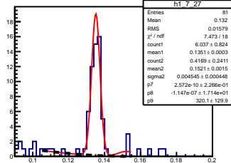
\pi^0 angle: [0.70, 0.80] elasticity: [1.16, 1.17]
