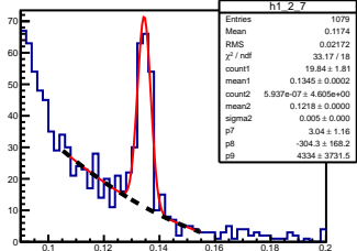
\pi^0 angle: [0.20, 0.30] elasticity: [0.89, 0.91]
