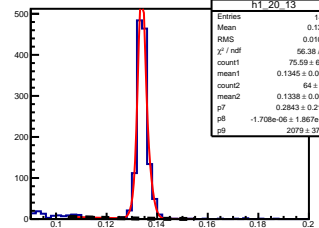
\pi^0 angle: [2.00, 2.10] elasticity: [0.97, 0.99]
