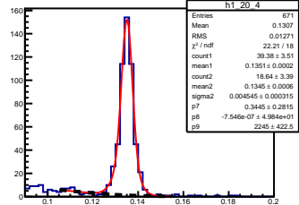
\pi^0 angle: [2.00, 2.10] elasticity: [0.85, 0.87]
