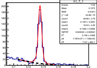
\pi^0 angle: [0.70, 0.80] elasticity: [0.81, 0.83]
