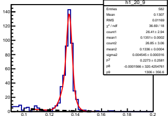
\pi^0 angle: [2.00, 2.10] elasticity: [0.92, 0.93]
