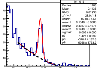
\pi^0 angle: [0.00, 0.10] elasticity: [0.87, 0.88]
