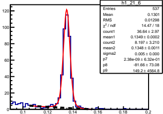
\pi^0 angle: [2.10, 2.20] elasticity: [0.88, 0.89]
