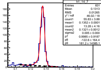
\pi^0 angle: [1.40, 1.50] elasticity: [0.89, 0.91]
