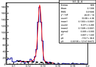
\pi^0 angle: [0.90, 1.00] elasticity: [0.85, 0.87]
