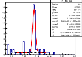
\pi^0 angle: [1.00, 1.10] elasticity: [1.17, 1.19]
