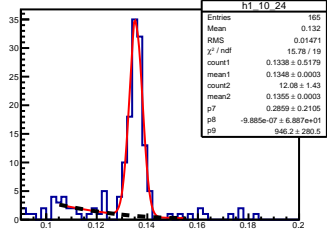
\pi^0 angle: [1.00, 1.10] elasticity: [1.12, 1.13]
