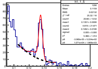
\pi^0 angle: [0.10, 0.20] elasticity: [0.87, 0.88]
