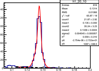
\pi^0 angle: [2.00, 2.10] elasticity: [0.93, 0.95]
