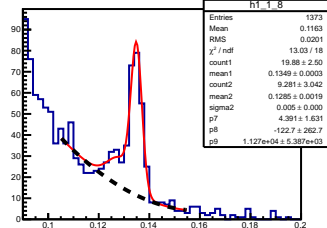
\pi^0 angle: [0.10, 0.20] elasticity: [0.91, 0.92]
