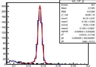
\pi^0 angle: [1.70, 1.80] elasticity: [0.84, 0.85]
