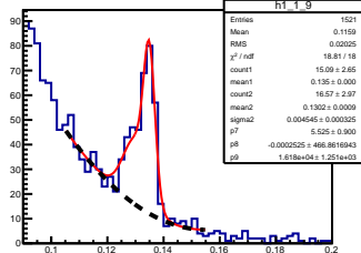
\pi^0 angle: [0.10, 0.20] elasticity: [0.92, 0.93]
