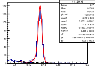
\pi^0 angle: [2.00, 2.10] elasticity: [0.88, 0.89]
