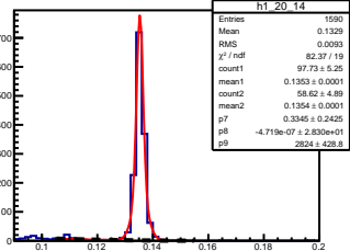
\pi^0 angle: [2.00, 2.10] elasticity: [0.99, 1.00]
