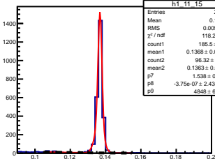
\pi^0 angle: [1.10, 1.20] elasticity: [1.00, 1.01]
