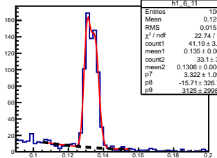
\pi^0 angle: [0.60, 0.70] elasticity: [0.95, 0.96]
