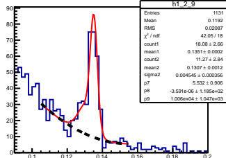
\pi^0 angle: [0.20, 0.30] elasticity: [0.92, 0.93]
