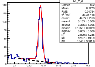
\pi^0 angle: [0.70, 0.80] elasticity: [0.88, 0.89]
