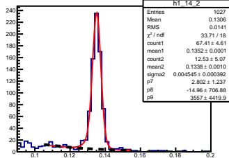
\pi^0 angle: [1.40, 1.50] elasticity: [0.83, 0.84]
