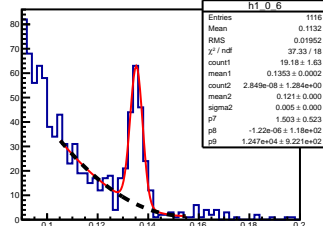
\pi^0 angle: [0.00, 0.10] elasticity: [0.88, 0.89]
