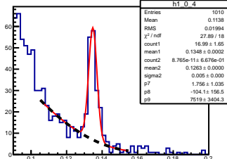
\pi^0 angle: [0.00, 0.10] elasticity: [0.85, 0.87]
