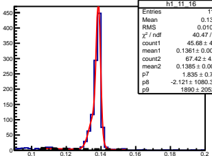
\pi^0 angle: [1.10, 1.20] elasticity: [1.01, 1.03]
