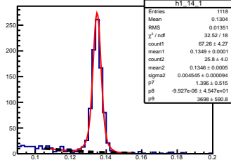
\pi^0 angle: [1.40, 1.50] elasticity: [0.81, 0.83]
