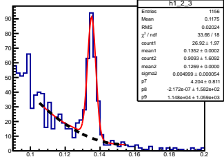
\pi^0 angle: [0.20, 0.30] elasticity: [0.84, 0.85]
