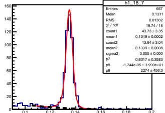
\pi^0 angle: [1.80, 1.90] elasticity: [0.89, 0.91]
