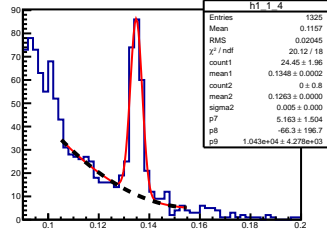
\pi^0 angle: [0.10, 0.20] elasticity: [0.85, 0.87]
