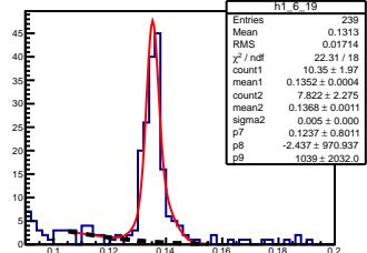
\pi^0 angle: [0.60, 0.70] elasticity: [1.05, 1.07]
