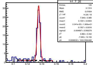
\pi^0 angle: [0.70, 0.80] elasticity: [1.13, 1.15]
