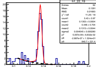
\pi^0 angle: [2.20, 2.30] elasticity: [1.05, 1.07]
