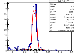
\pi^0 angle: [2.00, 2.10] elasticity: [1.03, 1.04]
