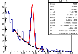
\pi^0 angle: [0.10, 0.20] elasticity: [0.84, 0.85]
