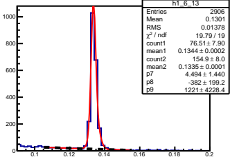
\pi^0 angle: [0.60, 0.70] elasticity: [0.97, 0.99]
