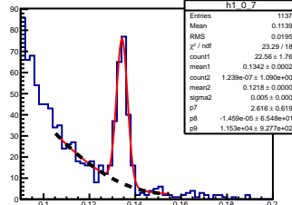
\pi^0 angle: [0.00, 0.10] elasticity: [0.89, 0.91]
