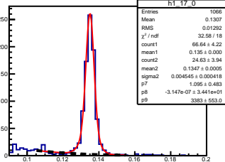
\pi^0 angle: [1.70, 1.80] elasticity: [0.80, 0.81]
