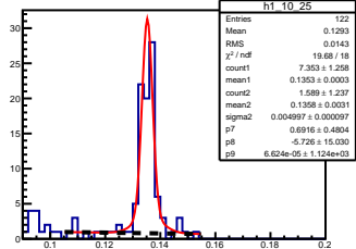
\pi^0 angle: [1.00, 1.10] elasticity: [1.13, 1.15]
