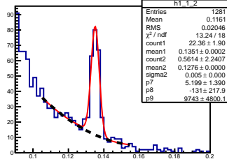
\pi^0 angle: [0.10, 0.20] elasticity: [0.83, 0.84]
