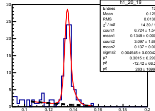
\pi^0 angle: [2.00, 2.10] elasticity: [1.05, 1.07]
