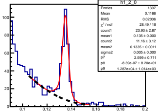
\pi^0 angle: [0.20, 0.30] elasticity: [0.80, 0.81]
