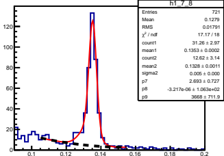
\pi^0 angle: [0.70, 0.80] elasticity: [0.91, 0.92]
