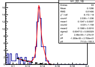
\pi^0 angle: [2.20, 2.30] elasticity: [1.04, 1.05]
