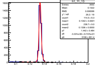
\pi^0 angle: [1.10, 1.20] elasticity: [0.97, 0.99]
