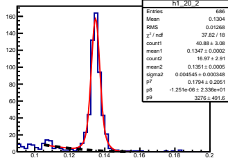
\pi^0 angle: [2.00, 2.10] elasticity: [0.83, 0.84]
