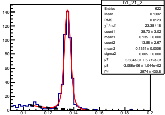
\pi^0 angle: [2.10, 2.20] elasticity: [0.83, 0.84]
