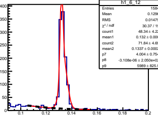
\pi^0 angle: [0.60, 0.70] elasticity: [0.96, 0.97]
