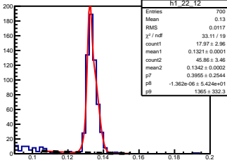
\pi^0 angle: [2.20, 2.30] elasticity: [0.96, 0.97]
