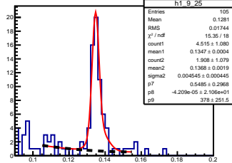
\pi^0 angle: [0.90, 1.00] elasticity: [1.13, 1.15]
