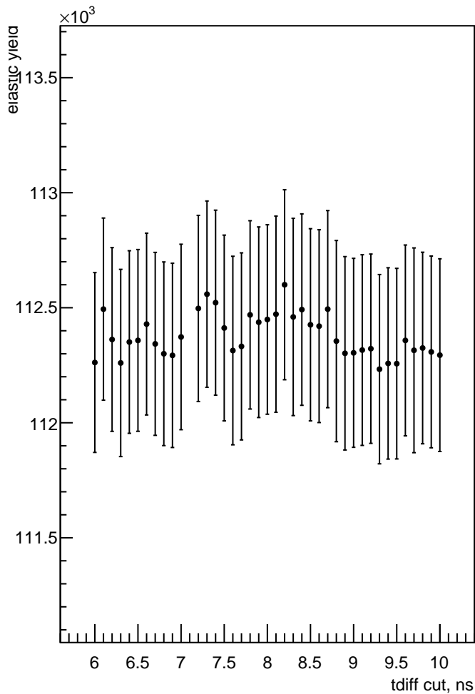
c12: elastic yield vs. tdiff cut (PbWO 4 acceptance)
