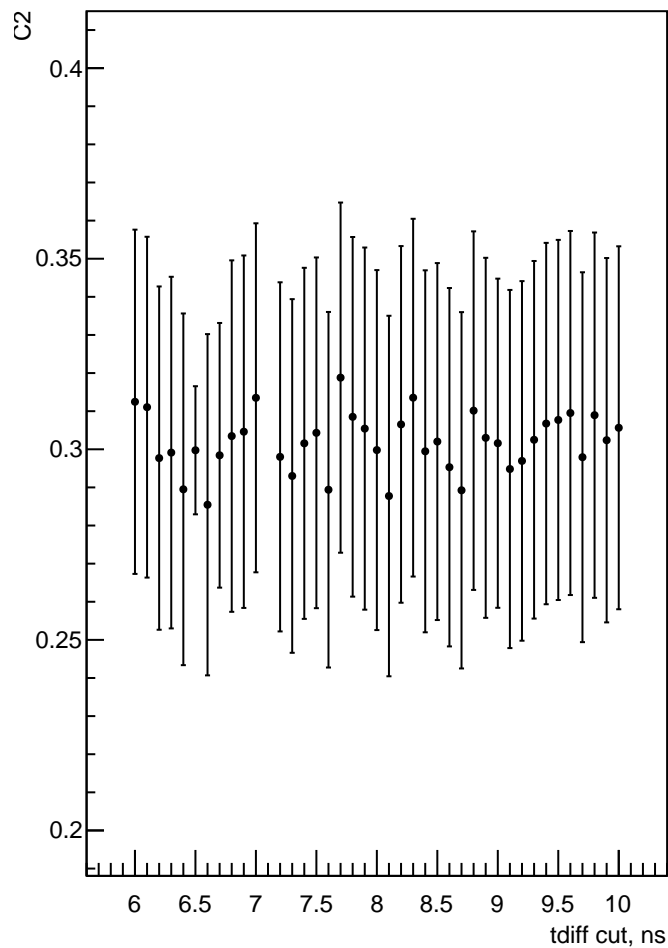
c12: C2 vs. tdiff
