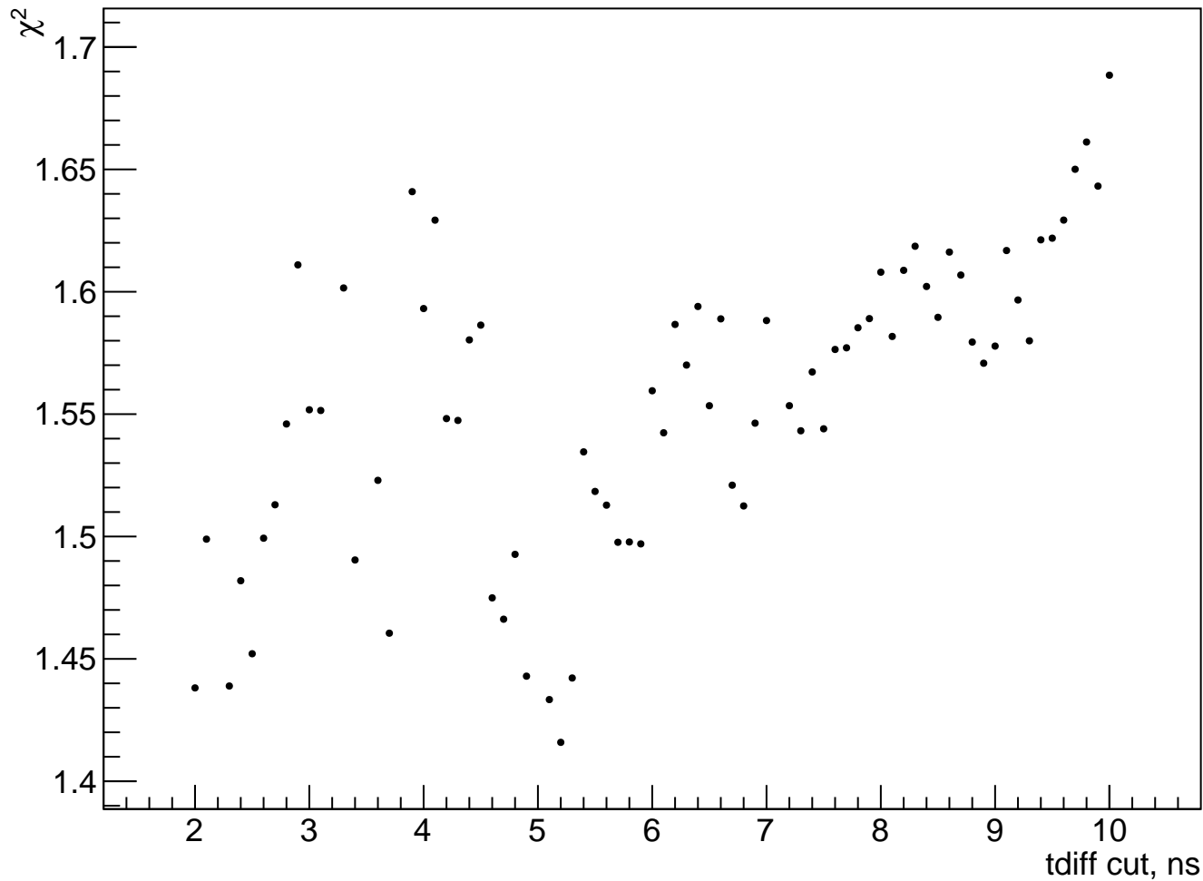
c12: yield fitting \chi^2 /NDF vs. tdiff cut
