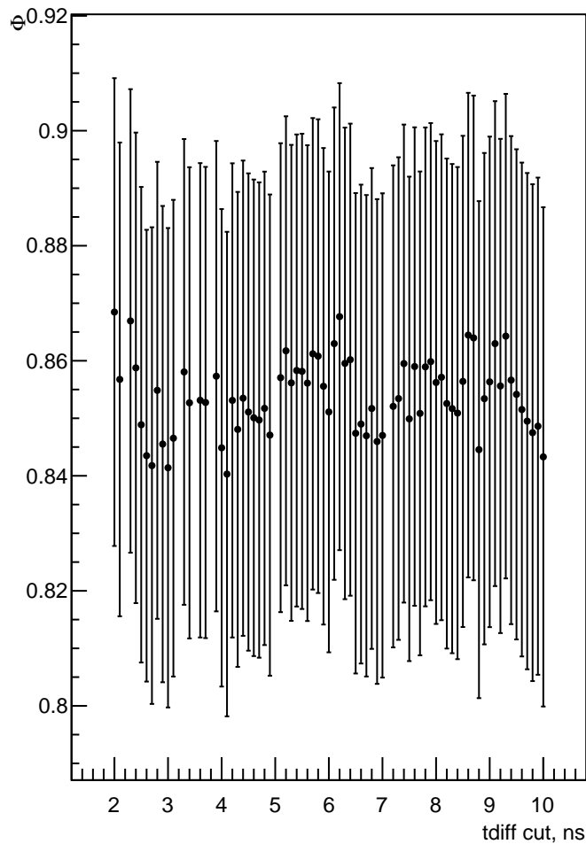
c12: \Phi vs. tdiff
