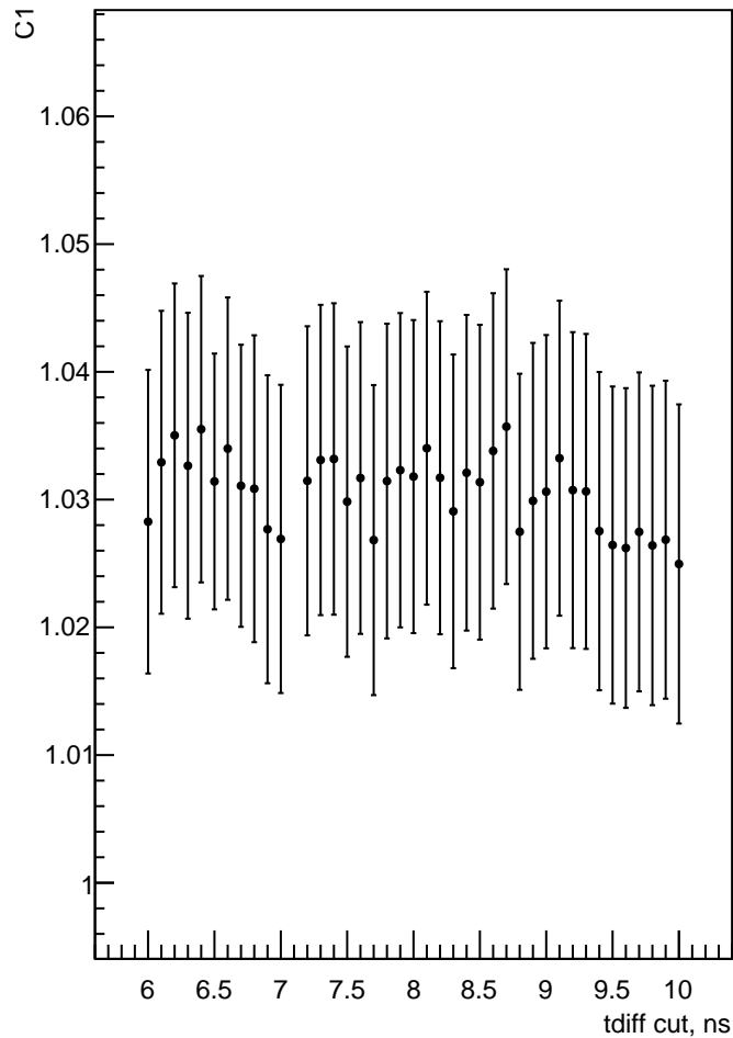
c12: C1 vs. tdiff
